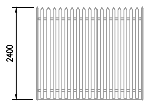
VIEW ON ARROW 'B'
